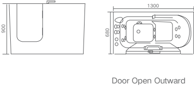
G9581 Size:1300x680x900mm Inner seat Water massage Bubble massage
