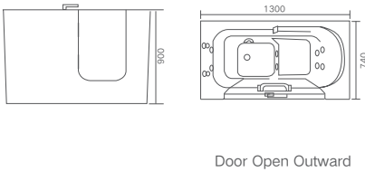
G9583 Size:1300x740x900mm Inner seat Water massage Bubble massage
