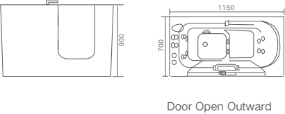
G9580 Size:1150x700x900mm Inner seat Water massage Bubble massage
