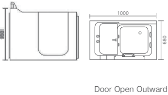
G9582 Size:1000x680x900mm Inner seat Water massage Bubble massage
