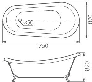
size:1750x820x820mm G9030-D
